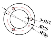
Flange details Scale 1:1
